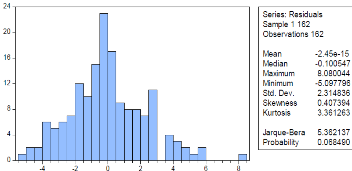
Figure 1. Normality Test
